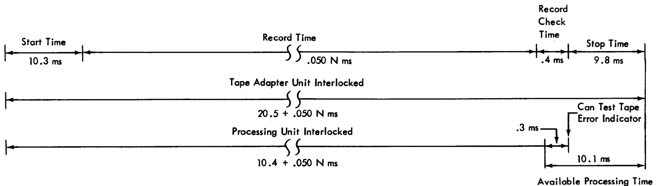
Figure 77. Read Operation Timing
