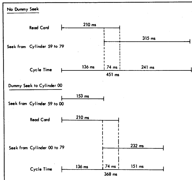
Figure 43. Throughput Time for Dummy Seek Technique
