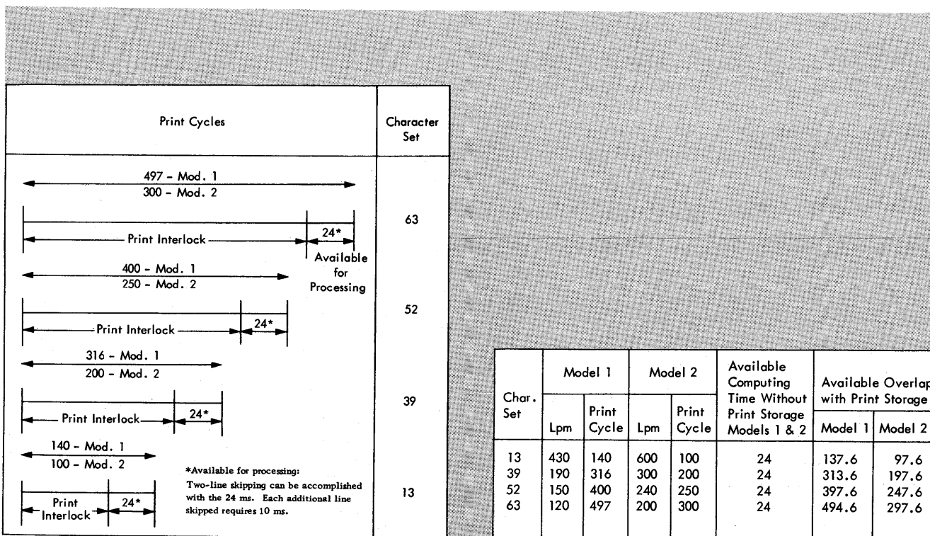
Figure 34. Print Cycles
