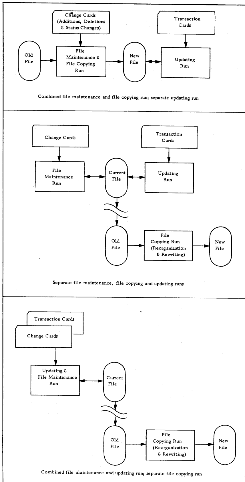
Figure 25. Relationship of File Maintenance, File Copying, and Updating Runs in Three File Maintenance Techniques
