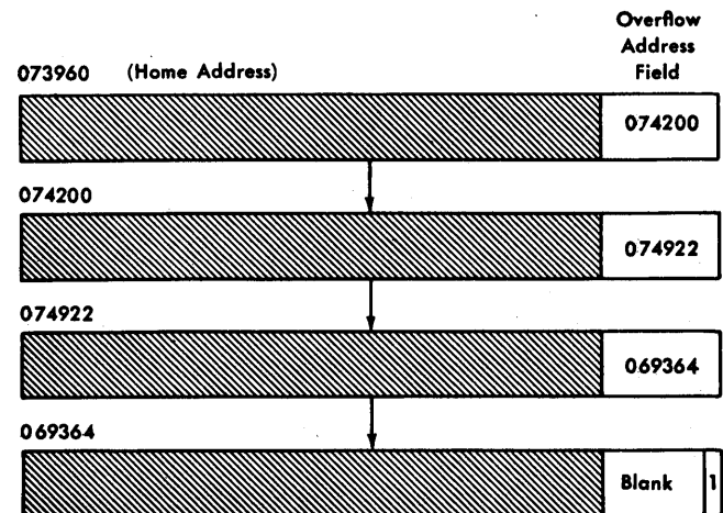
Figure 28. Example of Disk Storage Chaining
